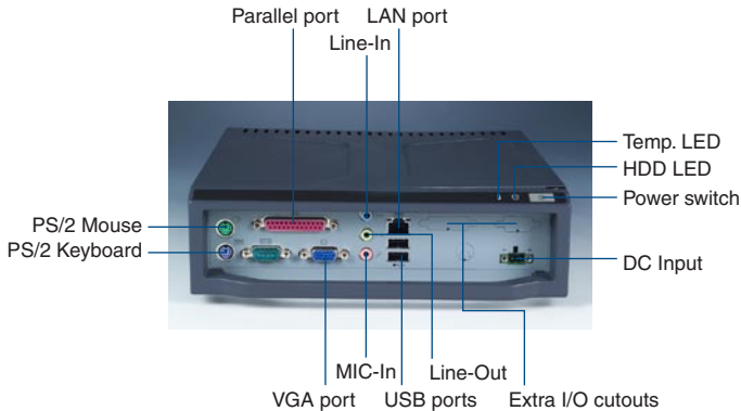
ARK-6310-3M01E/O2E Front IO view
