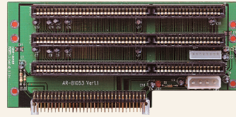
AR-B1053 PC/104 to ISA Transfer Board (3 Slots)
