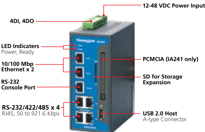
Serial Port, RJ45 Connector
