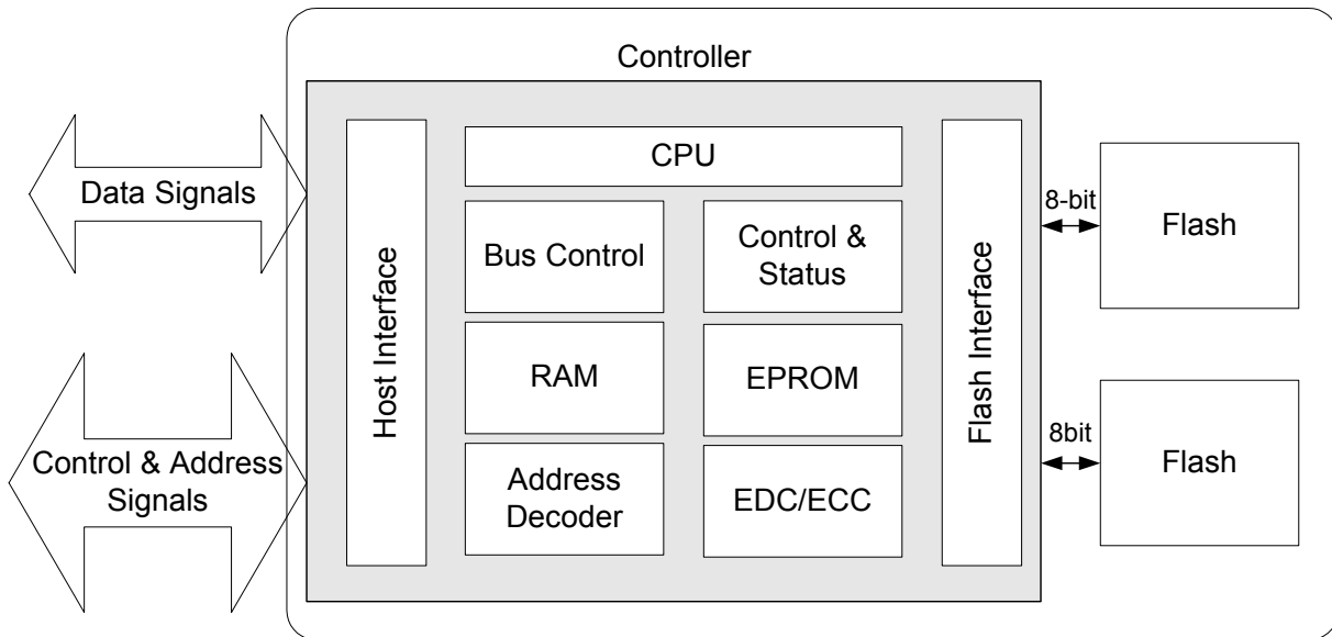
Figure 1: DiskOnChip IDE Pro Block Diagram
