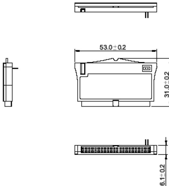
Figure 5: Dimensions of 44-Pin DiskOnChip IDE Pro
