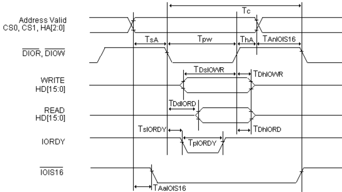
Figure 7: Timing Diagram, PIO Mode 4
