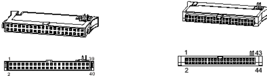
Figure 2: IDE Pro 44-pin (left) and 40-Pin (right) Connector Layouts
