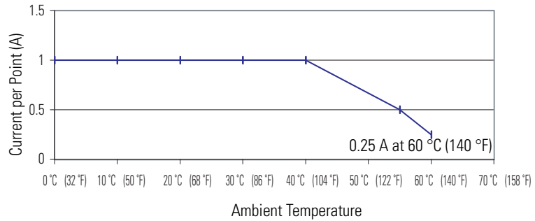
Current Derating Based on Temperature
