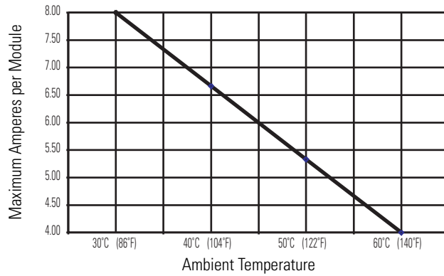
1769-OB32 Maximum Amperes per Module vs. Temperature
