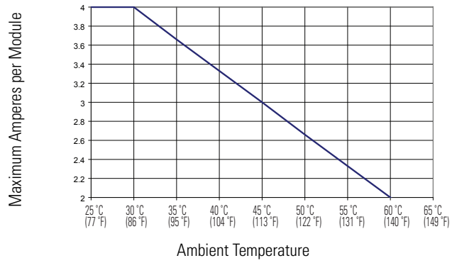
1769-BOOLEAN Maximum Amperes per Module versus Temperature
