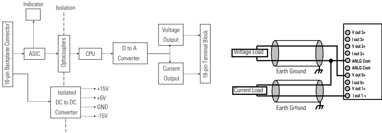
Simplified Schematic
