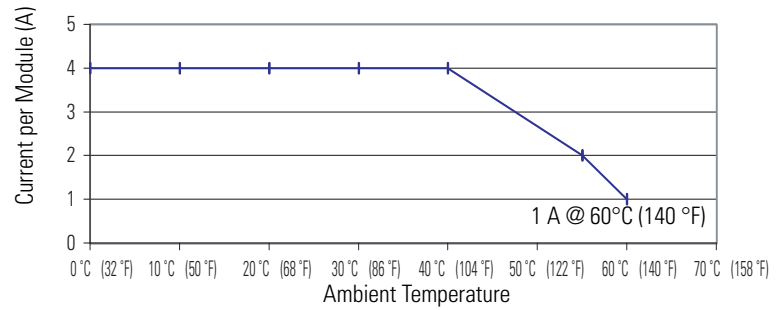
Current Derating Based on Temperature
