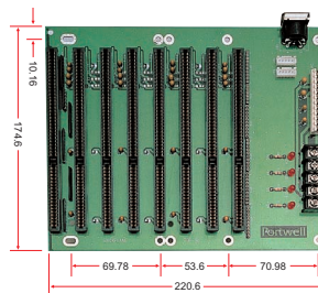
8-slot Passive ISA Backplane
