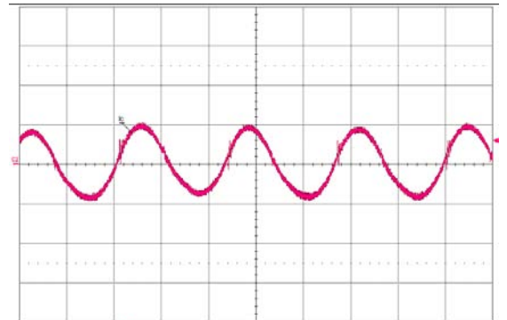
Figure 15. Input reflected ripple-current, i_C (100 mA/div.), measured at input terminals at full rated load current and V_{in} = 48\text{ V} . Refer to Fig. J for test setup. Time scale: 1 \mu\text{s} /div.
