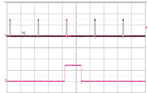
Figure 16. Load current (top trace, 20 A/div., 100 ms/div.) into a 10 \text{m}\Omega short circuit during restart, at V_{in} = 48\text{ V} . Bottom trace (20 A/div., 5 ms/div.) is an expansion of the on-time portion of the top trace.
