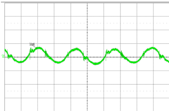
Figure 13. Output voltage ripple (20 mV/div.) at full rated load current into a resistive load with C_o = 10\mu\text{F} tantalum + 1 \mu\text{F} ceramic and V_{in} = 48\text{ V} . Time scale: 1 \mu\text{s} /div.
