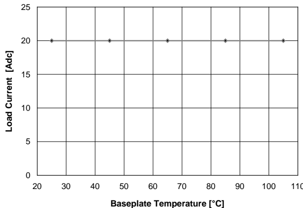
Figure 4. Coldplate cooling: Power derating of SQL48T20033-xxxBx converter with baseplate option and coldplate cooling. No thermal derating required. (Conditions: Air velocity \leq 30\text{ LFM} ( \leq 0.15\text{ m/s} ), V_{in} = 48\text{ V} , T_B \leq 105^\circ\text{C} )
