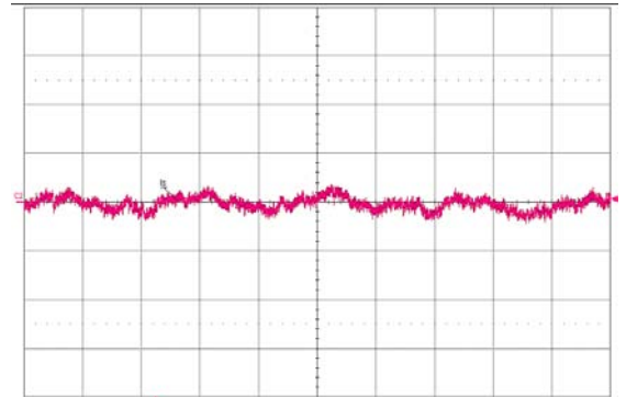
Figure 14. Input reflected-ripple current, i_S (10 mA/div.), measured through 10 \mu\text{H} at the source at full rated load current and V_{in} = 48\text{ V} . Refer to Fig. J for test setup. Time scale: 1 \mu\text{s} /div.
