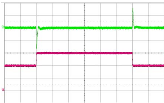
Figure 12. Output voltage response to load current step change (10A – 15A – 10A) at V_{in} = 48\text{ V} . Top trace: output voltage (50mV/div.) Bottom: load current (5 A/div.). Current slew rate: 1 A/ \mu\text{s} . Time scale: 200 \mu\text{s} /div. C_o = 470\mu\text{F} POS + 1 \mu\text{F} ceramic
