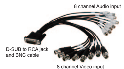
VIOCARD-GPIO (Optional)
