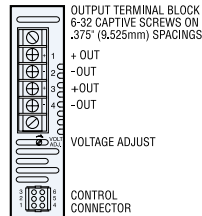
SINGLE WIDTH TYPE II BARRIER BLOCK
