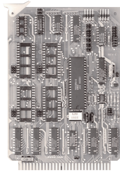
8085 CPU
