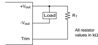
Fig. 8. Variable Trim
