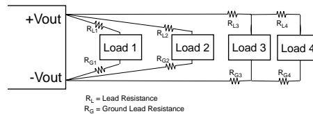
Fig. 20. Mixed Distribution
