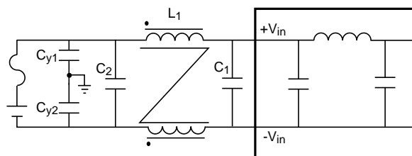
Fig. 5. EMI Reduction Input Filter
