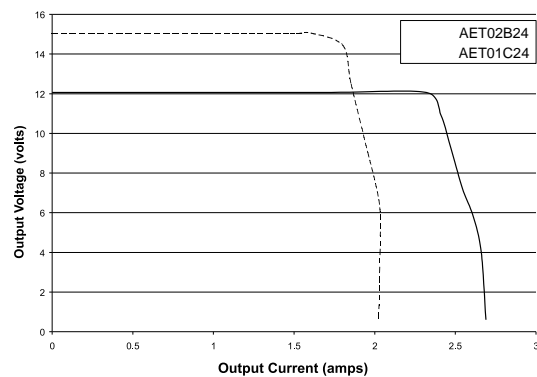
Fig. 7. Overcurrent Performance
