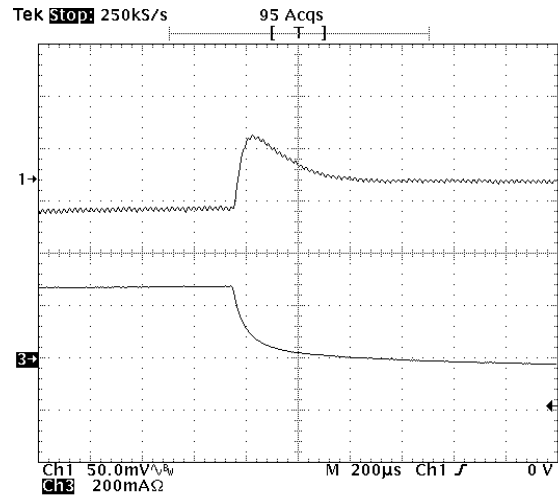
Typical step down load response from 50% to 25% load. AER01C24
