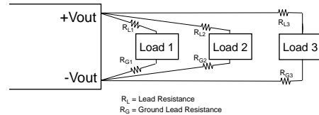
Fig. 19. Radial Distribution
