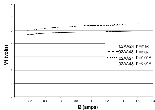
Fig. 6. Cross Regulation
