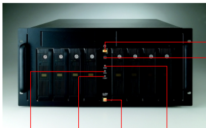
Fan LED TEMP LED Alarm reset switch Power LED
