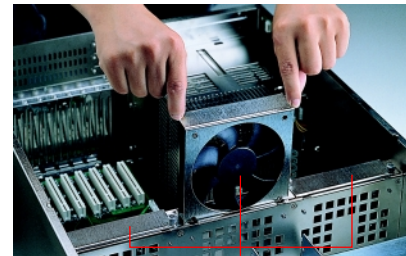
Three 114-CFM hot-swap cooling fans
