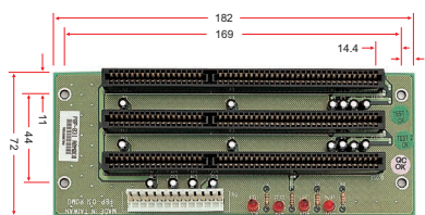
3-slot Passive ISA Backplane
