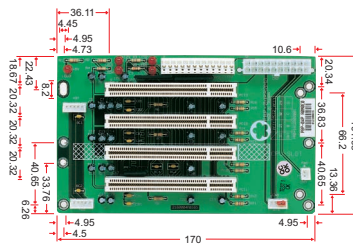
4-slot Passive PCI Backplane
