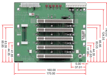
5-slot Passive PCI Backplane
