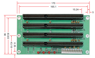
4-slot Passive ISA Backplane
